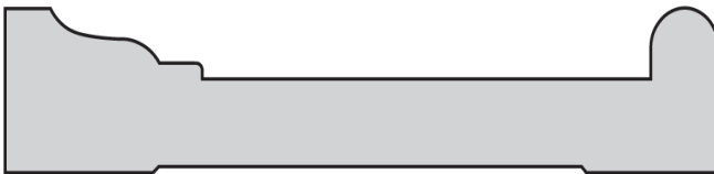
▲ FJP512HK 1-1/16" X 5-1/2" Casing
